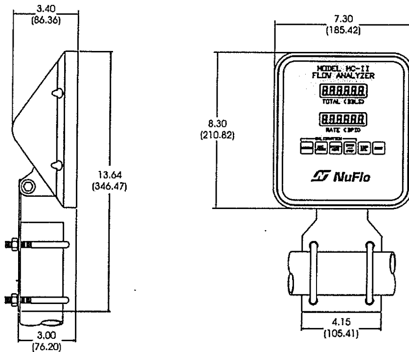
Figure 4—Remote mount dimensions (inches and millimeters) 10000 5129
