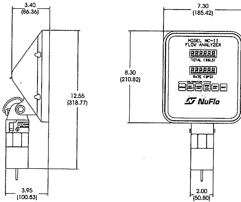
Figure 3—Direct mount dimensions (inches and millimeters) 10000 5130 100.
